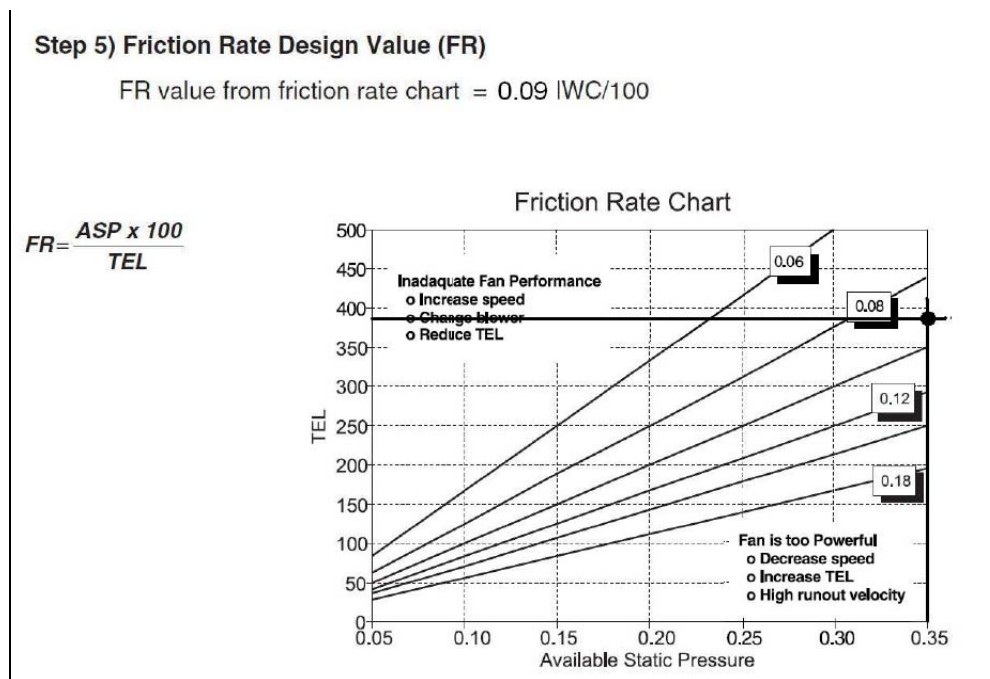
Figure 18: Friction Rate Worksheet - Bottom Section
